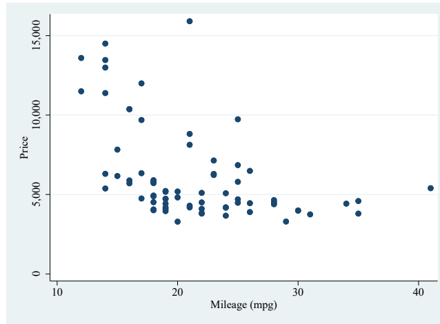
Figure 1: A scatterplot.
